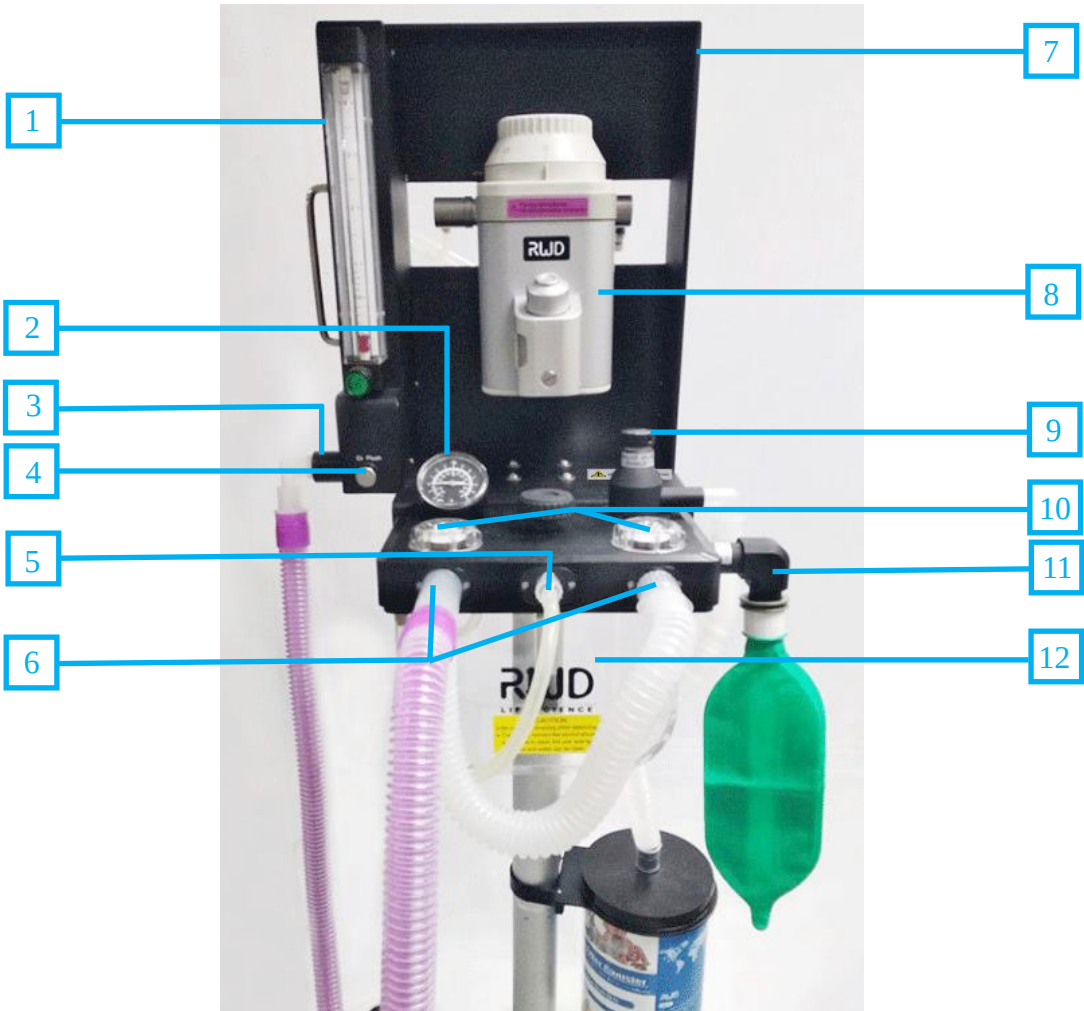
Figure 1-1 R620-MRI body
